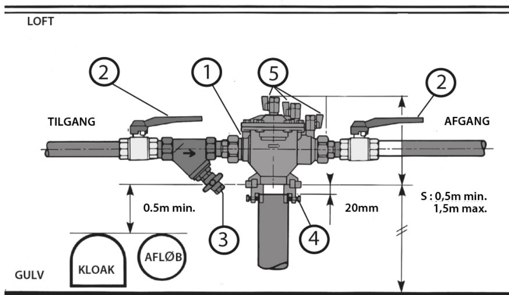
Fig. Installationstegning
