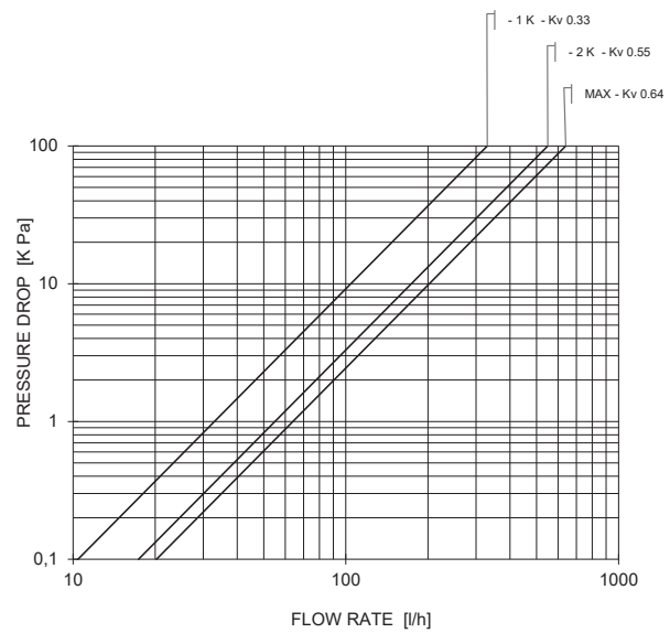
Right-angle with actuator 148WM, 148SDWM, 148CDWM 179WM DN 1/2"
