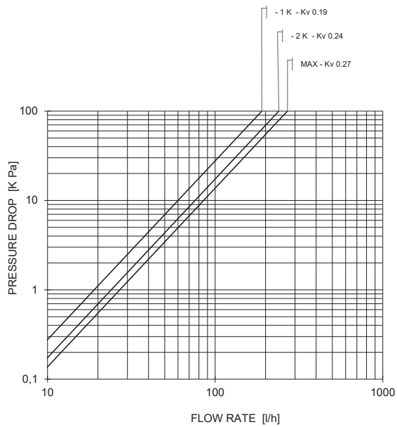
Right-angle with actuator 148WM, 148SDWM, 148CDWM 179WM DN 1/2"
