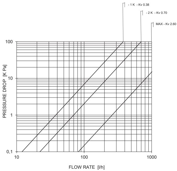
Right-angle body without pre-settings 178WM DN 1/2"
