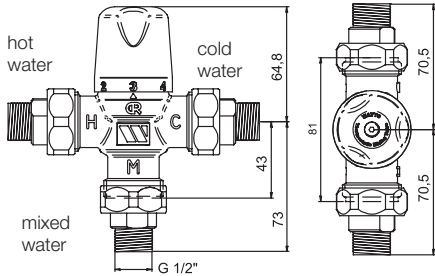
Connection union 1/2"
