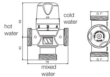
Thread 1"
